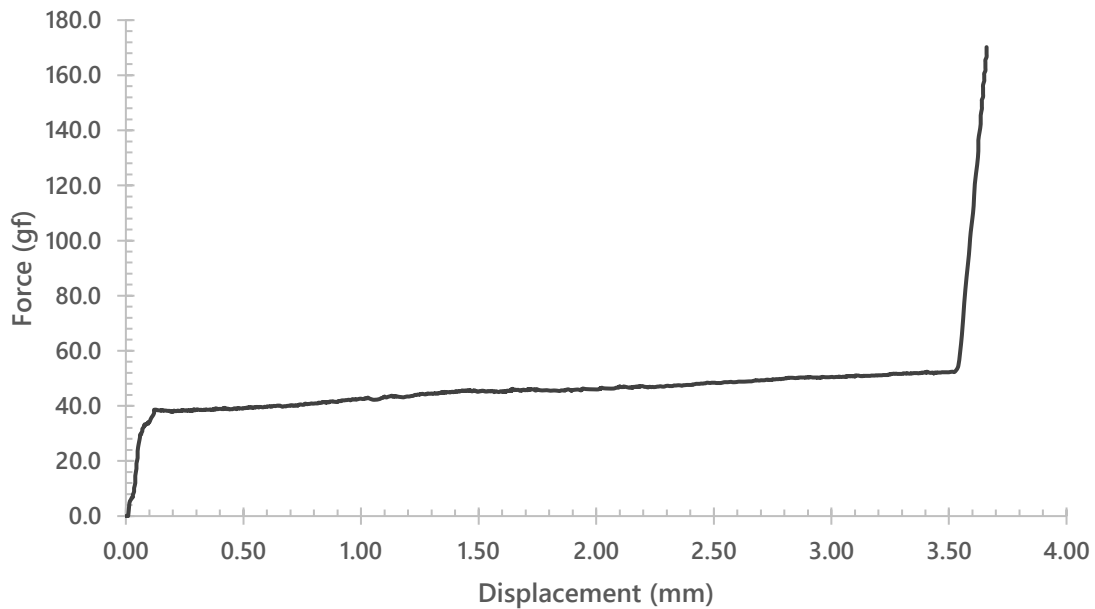
Kailh Mix-5 Red (Upstroke)
